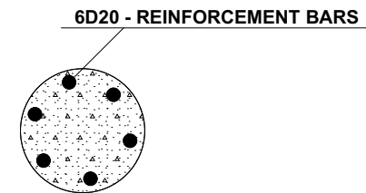
COLUMNS CROSS SECTION
